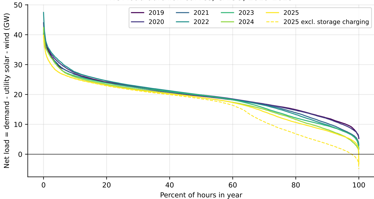
Net-load duration curves, CAISO, 2019-2025
