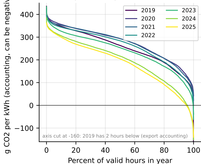
Hourly intensity duration curves
