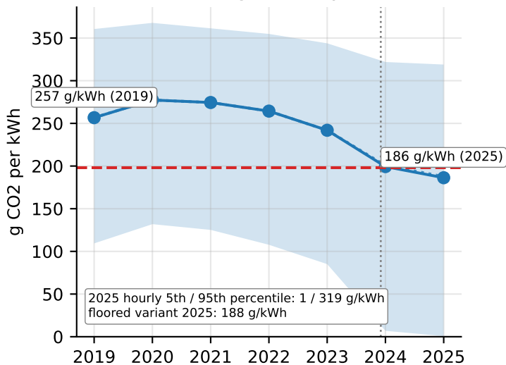
Annual CO2 accounting intensity of CAISO demand
