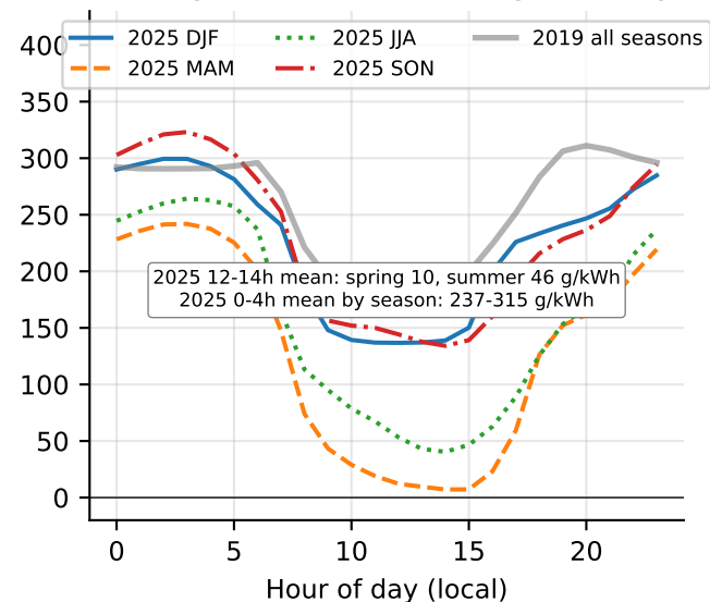
Average diurnal accounting intensity
