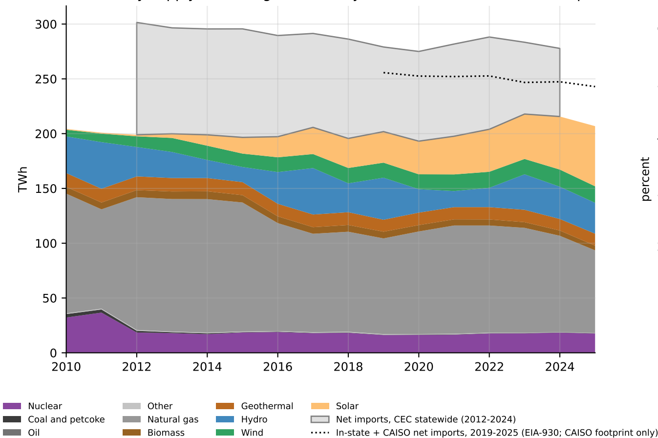
California electricity supply: in-state generation by resource (EIA-923) and net imports (CEC)
