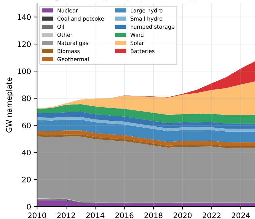
Operable capacity by technology (EIA-860)
