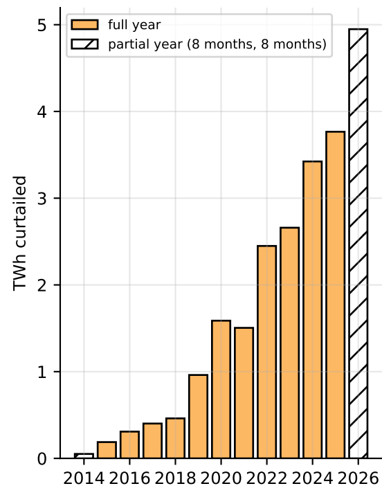
CAISO wind and solar curtailment
