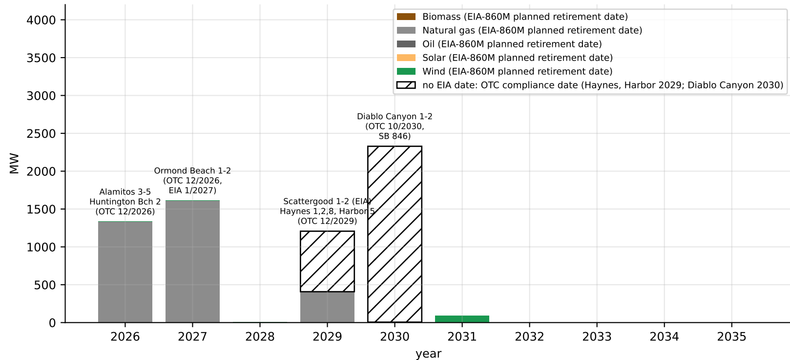
Scheduled retirements in California: EIA-860M planned dates and State Water Board once-through-cooling compliance dates
