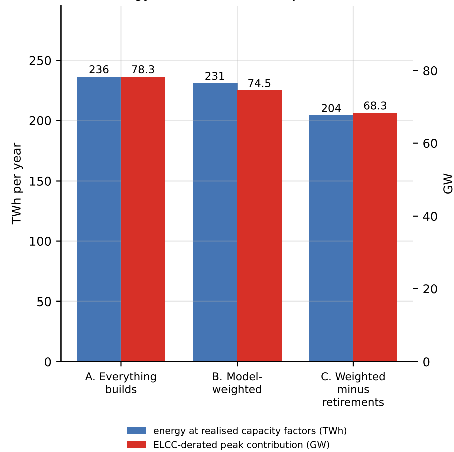
Energy and ELCC-derated peak, 2030
