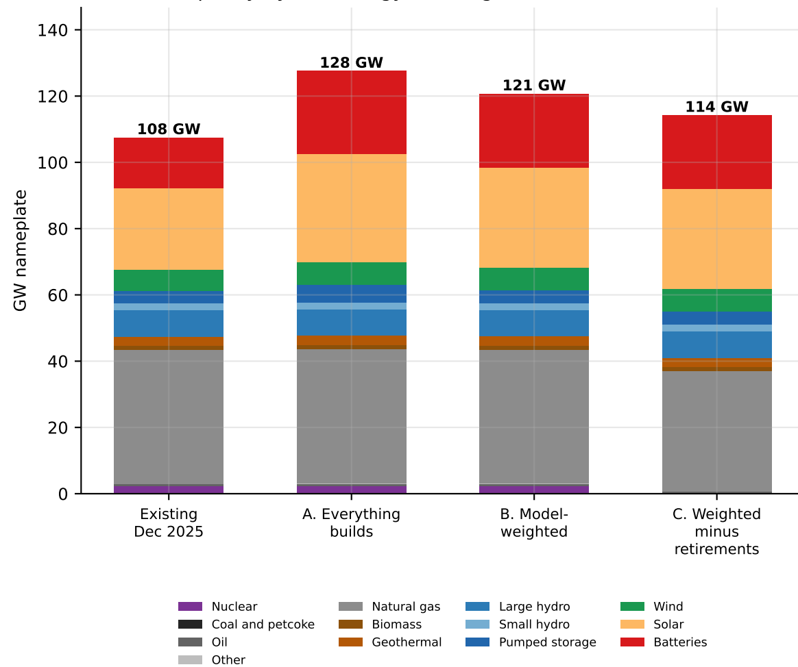
Capacity by technology: existing and three 2030 cases
