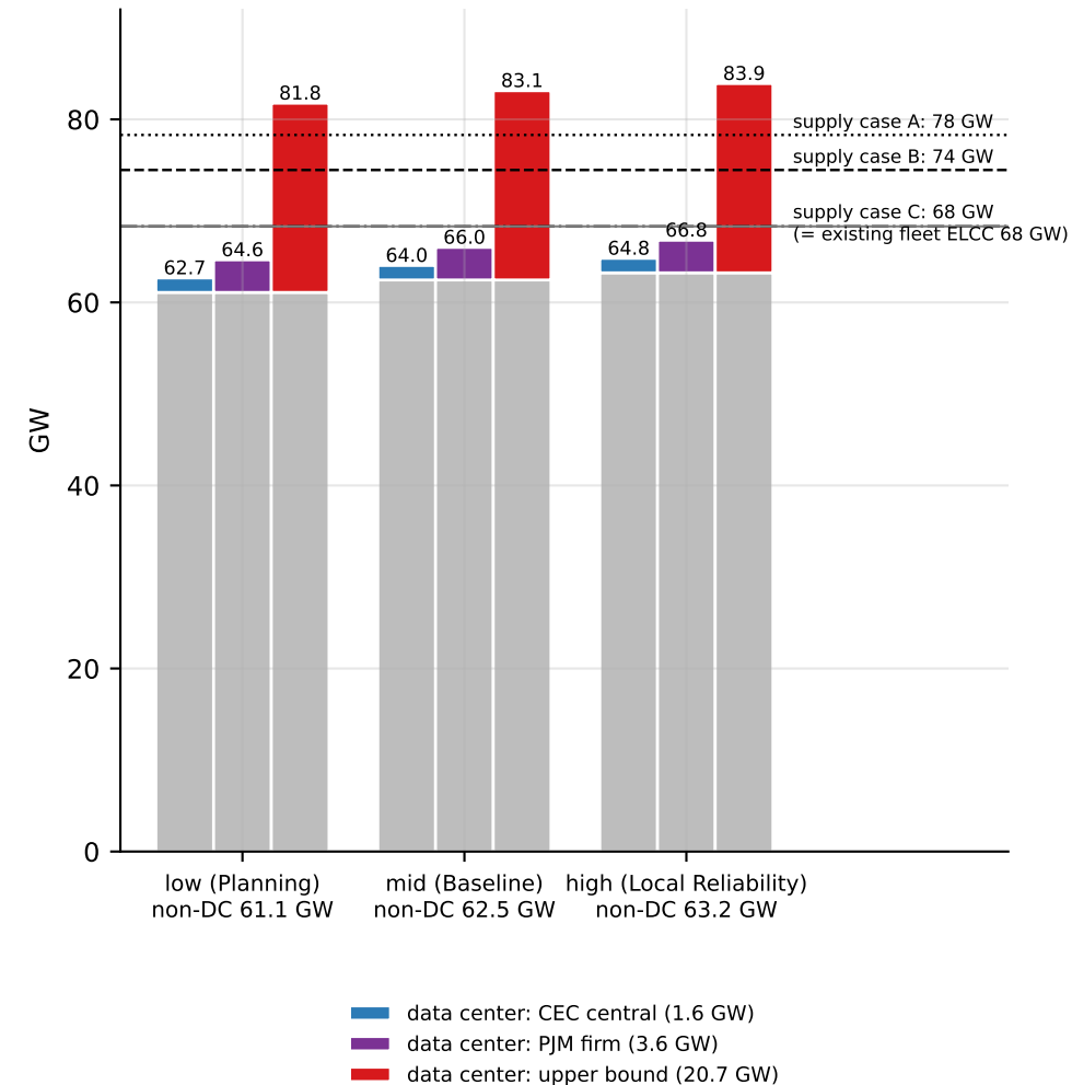
2030 statewide coincident peak by IEPR case (non-DC plus data centers) against ELCC-derated supply of Chapter 3
