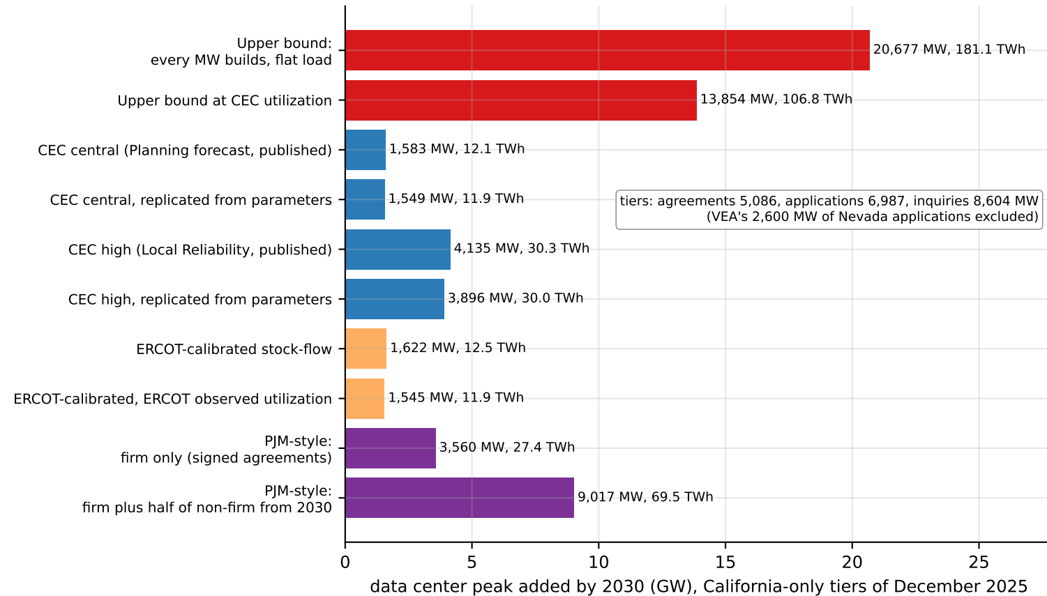
Data center demand in 2030 under each counting rule
