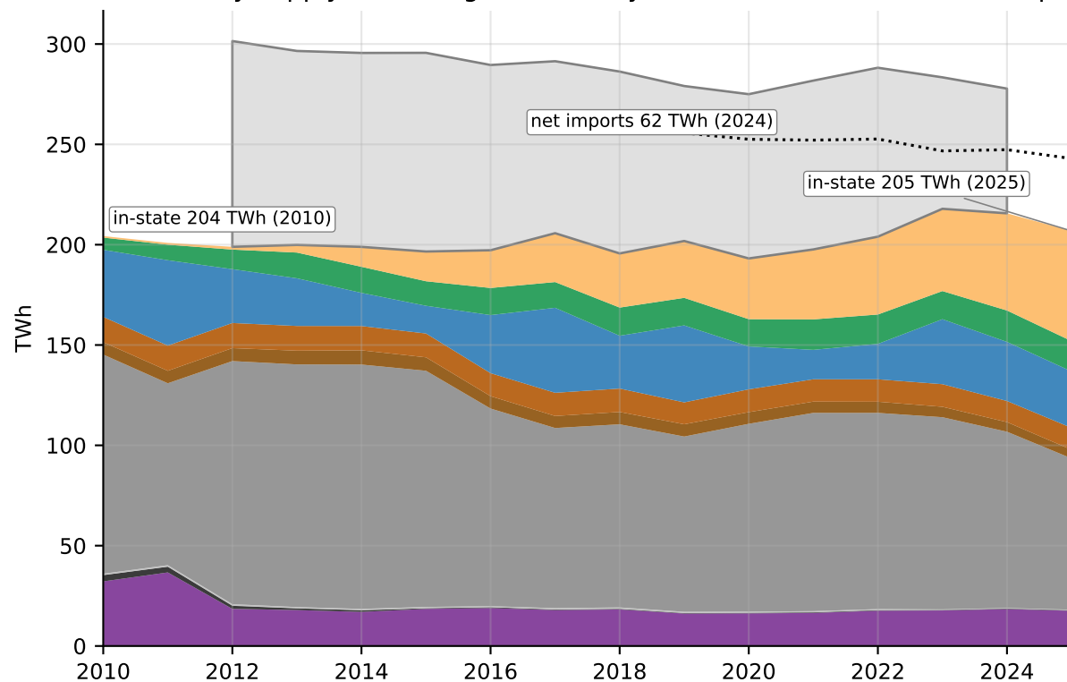
California electricity supply: in-state generation by resource (EIA-923) and net imports (CEC)
