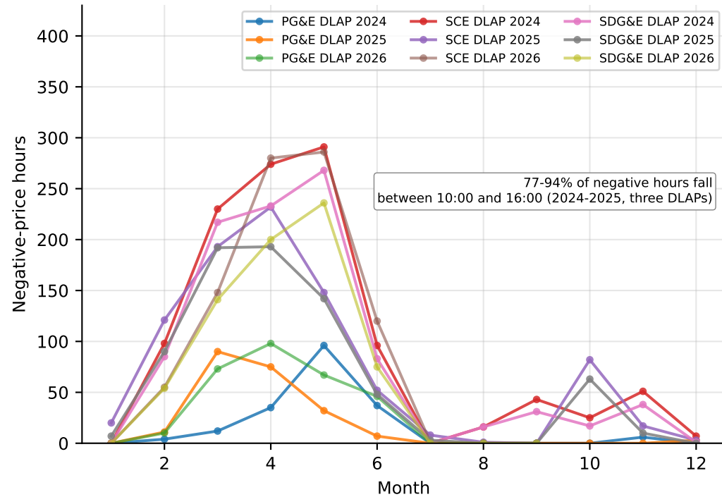
Negative-price hours by month
