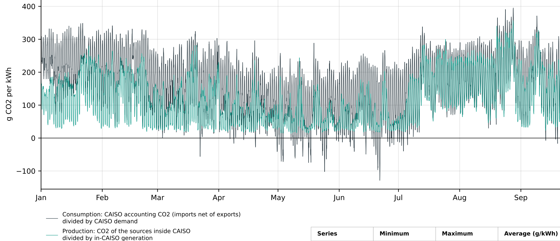
CAISO hourly CO2 intensity, January 1 to September 20, 2026: consumption (accounting) and production factors (CAISO Today's Outlook)
