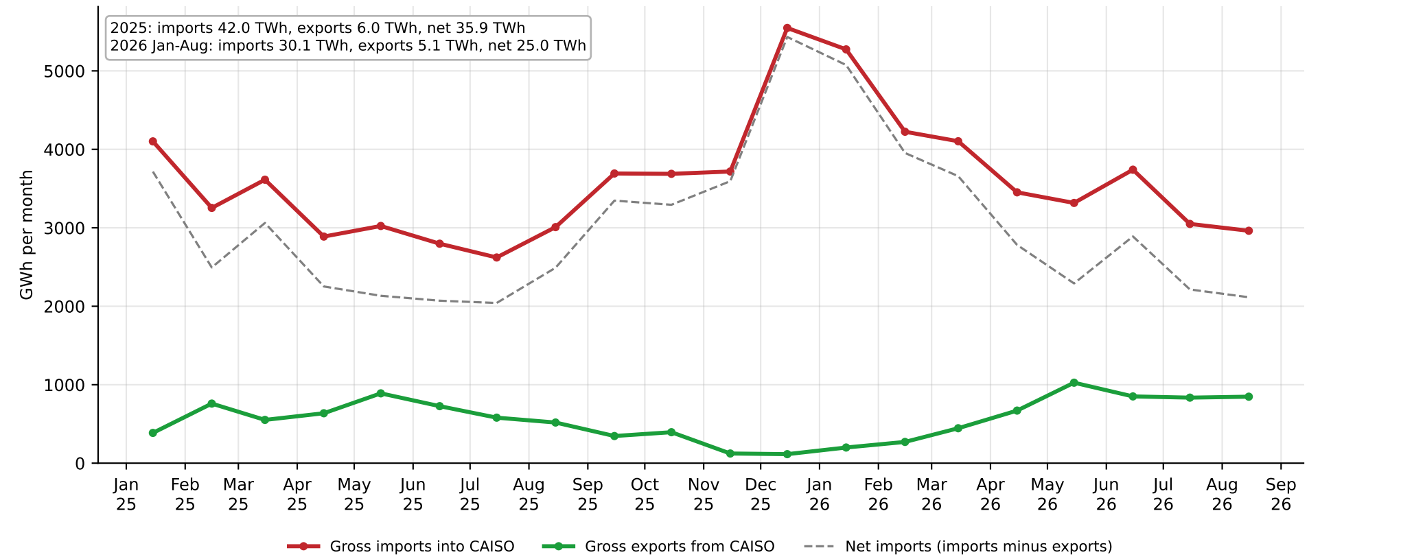
CAISO gross imports and exports by month, January 2025 to August 2026 (EIA-930 interchange with each neighbouring balancing authority; complete months)
