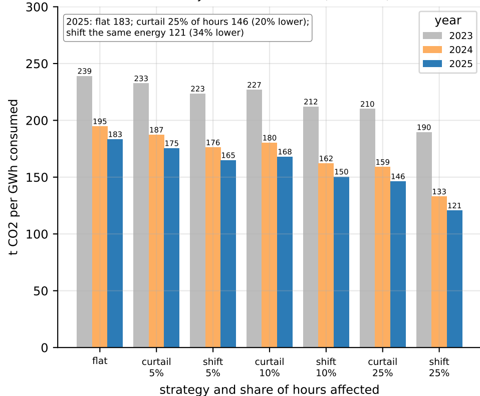
Emissions intensity of a 1 MW load: flat, curtailed, or shifted
