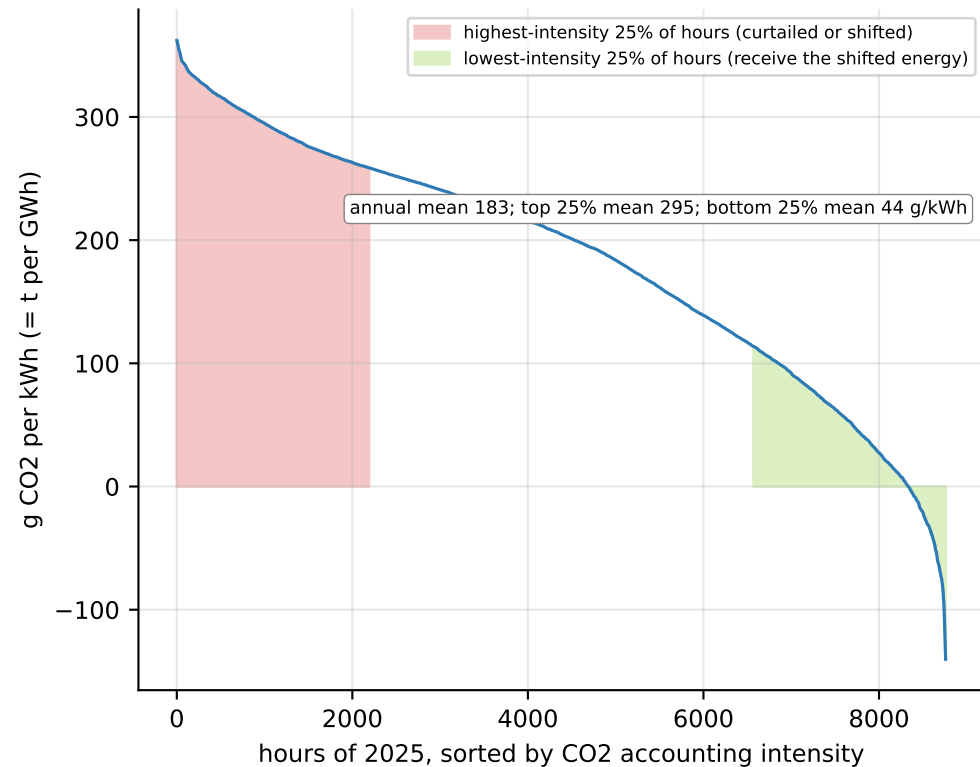
CAISO hourly intensity, 2025
