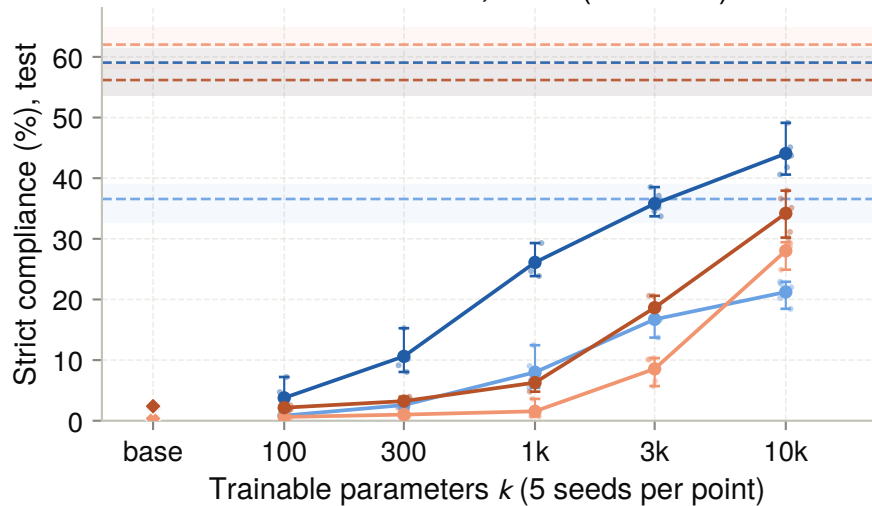
(c) Few-shot traces, main (9 modes)
