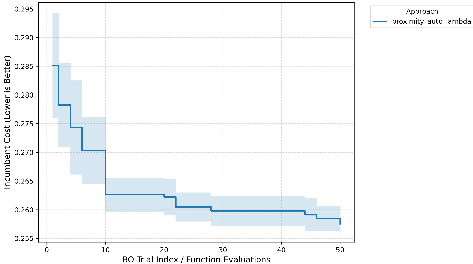
Anytime Performance: cfg_ml_svm_31
