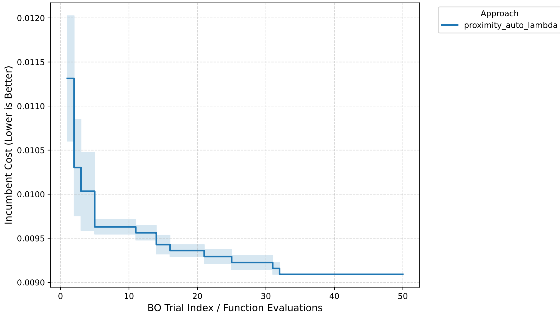
Anytime Performance: cfg_ml_xgboost_12
