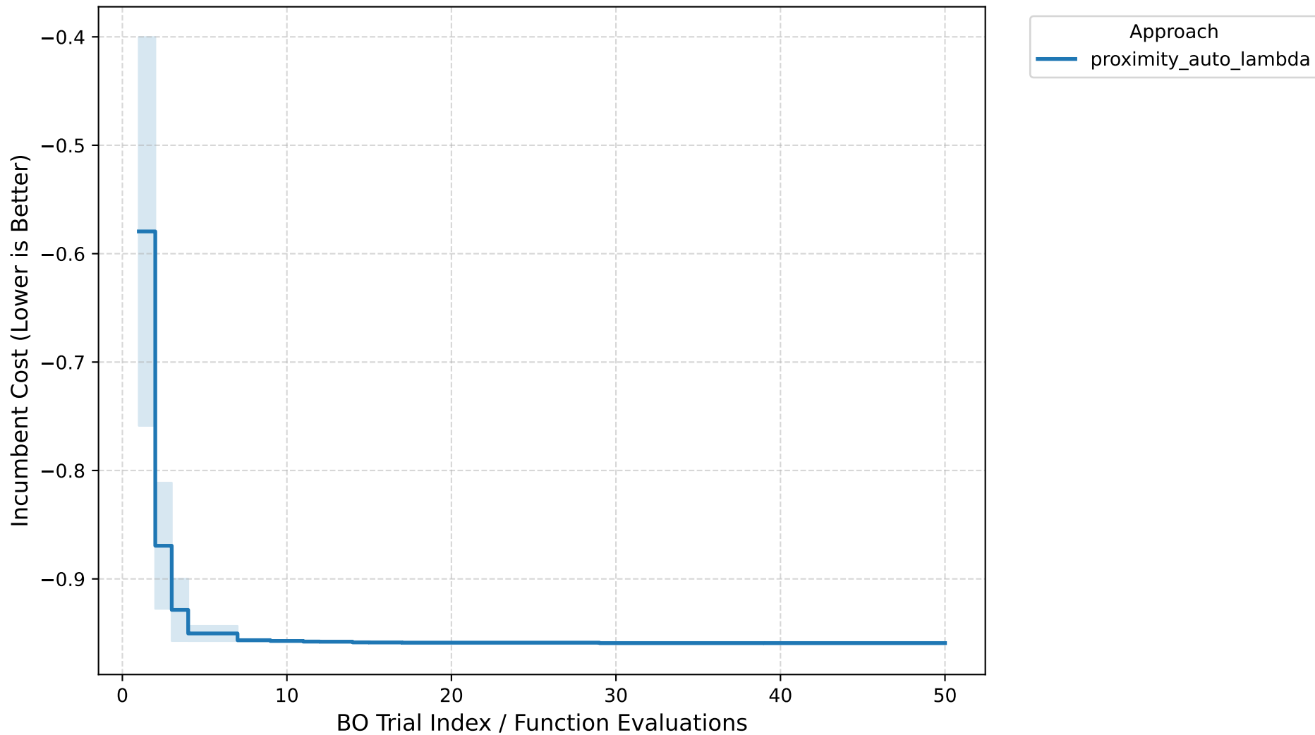
Anytime Performance: cfg_rbv2_glmnet_375
