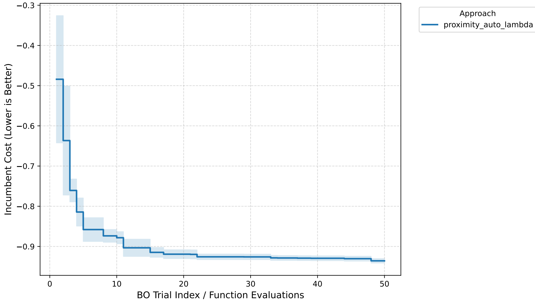
Anytime Performance: cfg_rbv2_xgboost_1501
