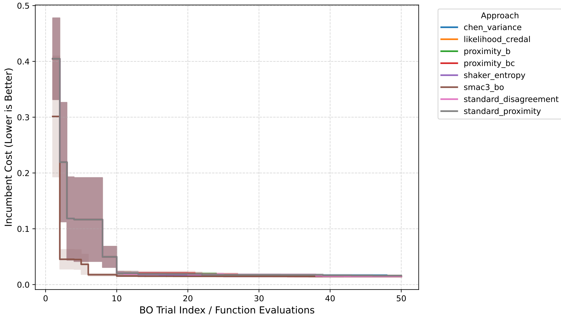
Anytime Performance: cfg_ml_svm_3
