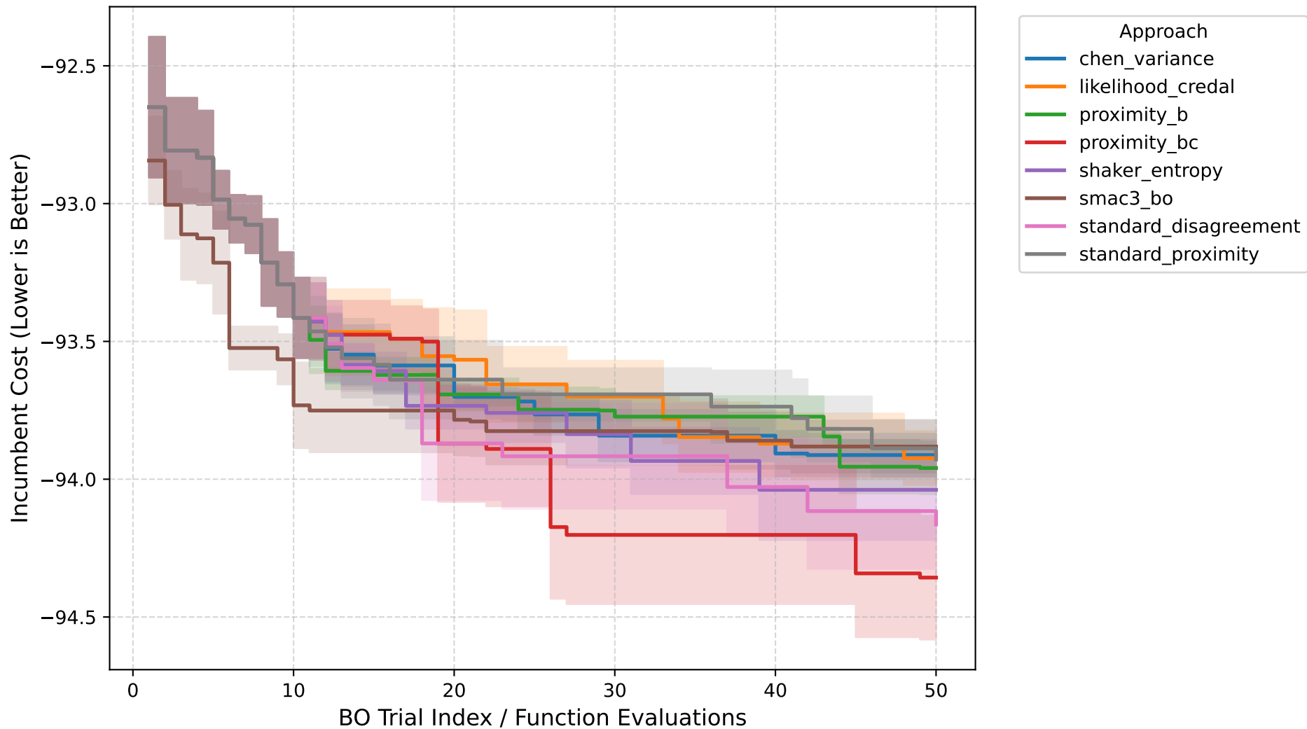
Anytime Performance: cfg_nb301_CIFAR10
