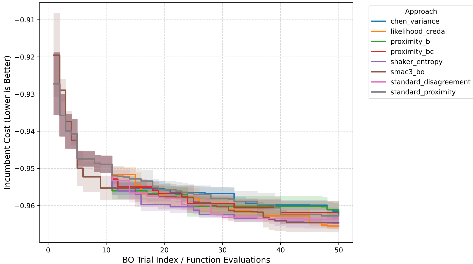
Anytime Performance: cfg_rbv2_ranger_16
