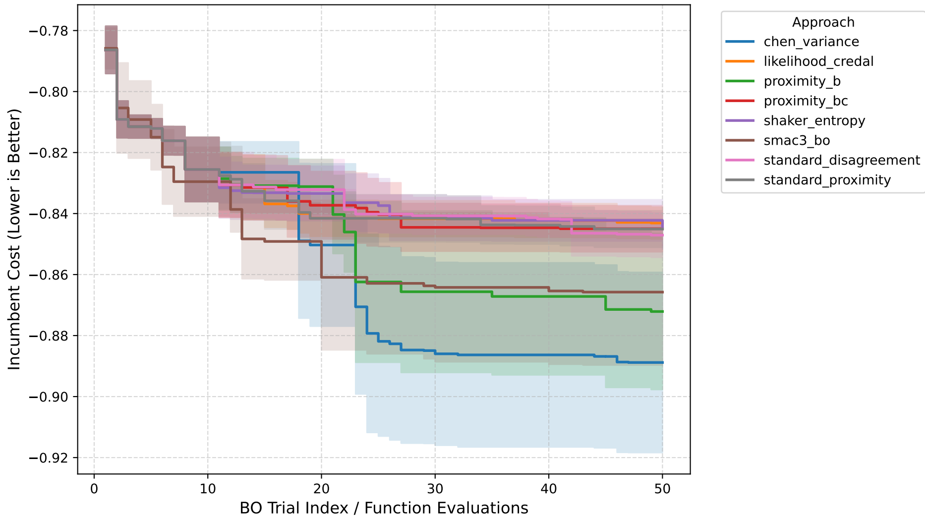
Anytime Performance: cfg_rbv2_super_1053
