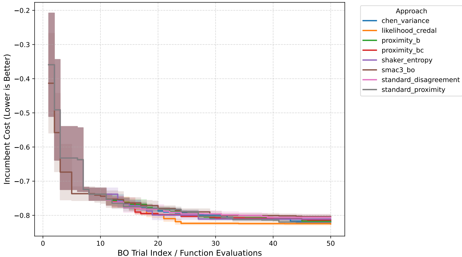
Anytime Performance: cfg_rbv2_super_1457
