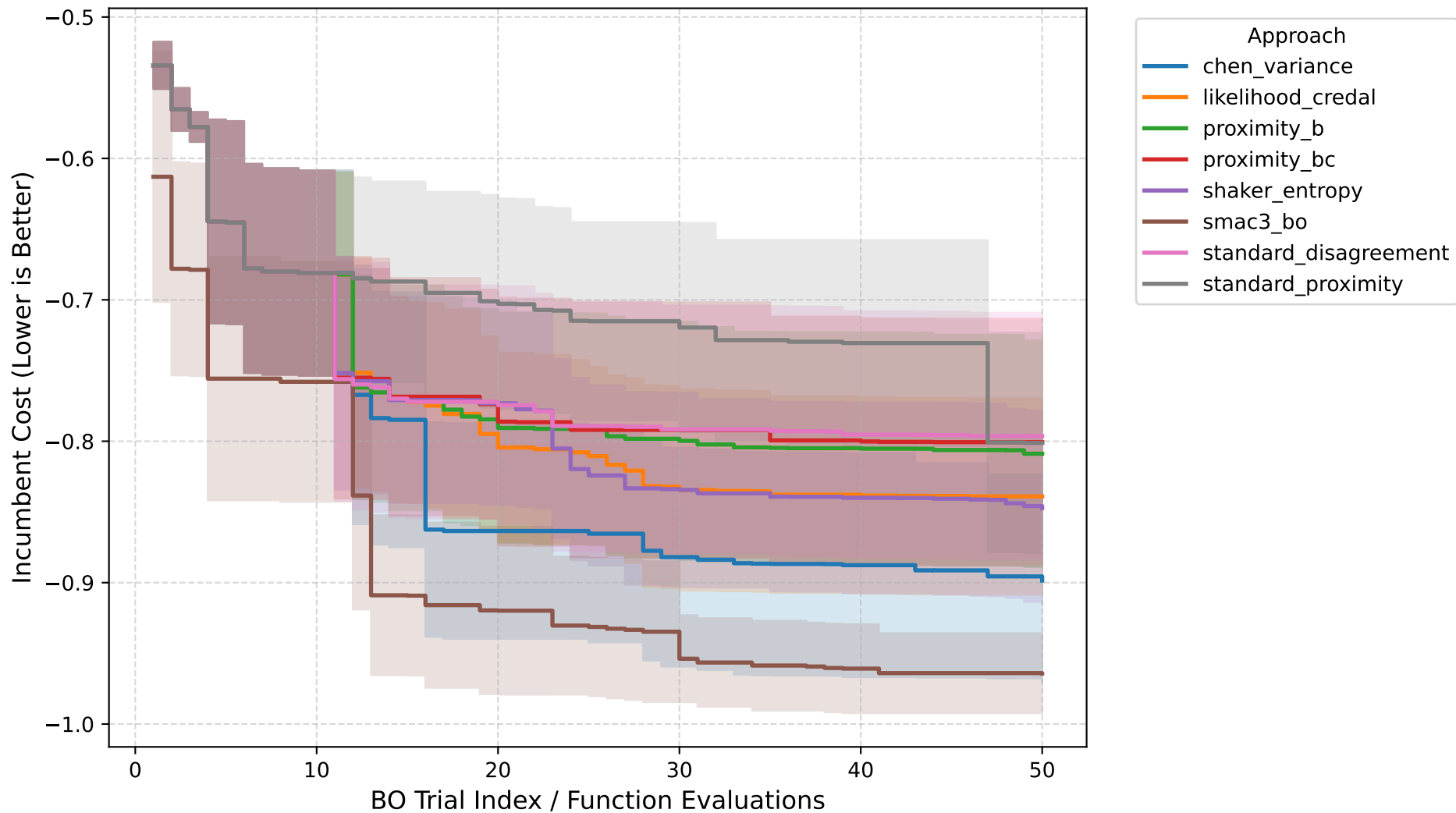
Anytime Performance: cfg_rbv2_super_1479
