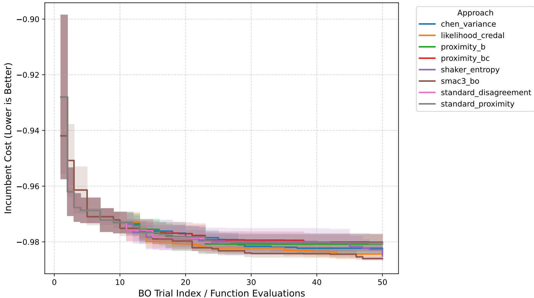
Anytime Performance: cfg_rbv2_super_15
