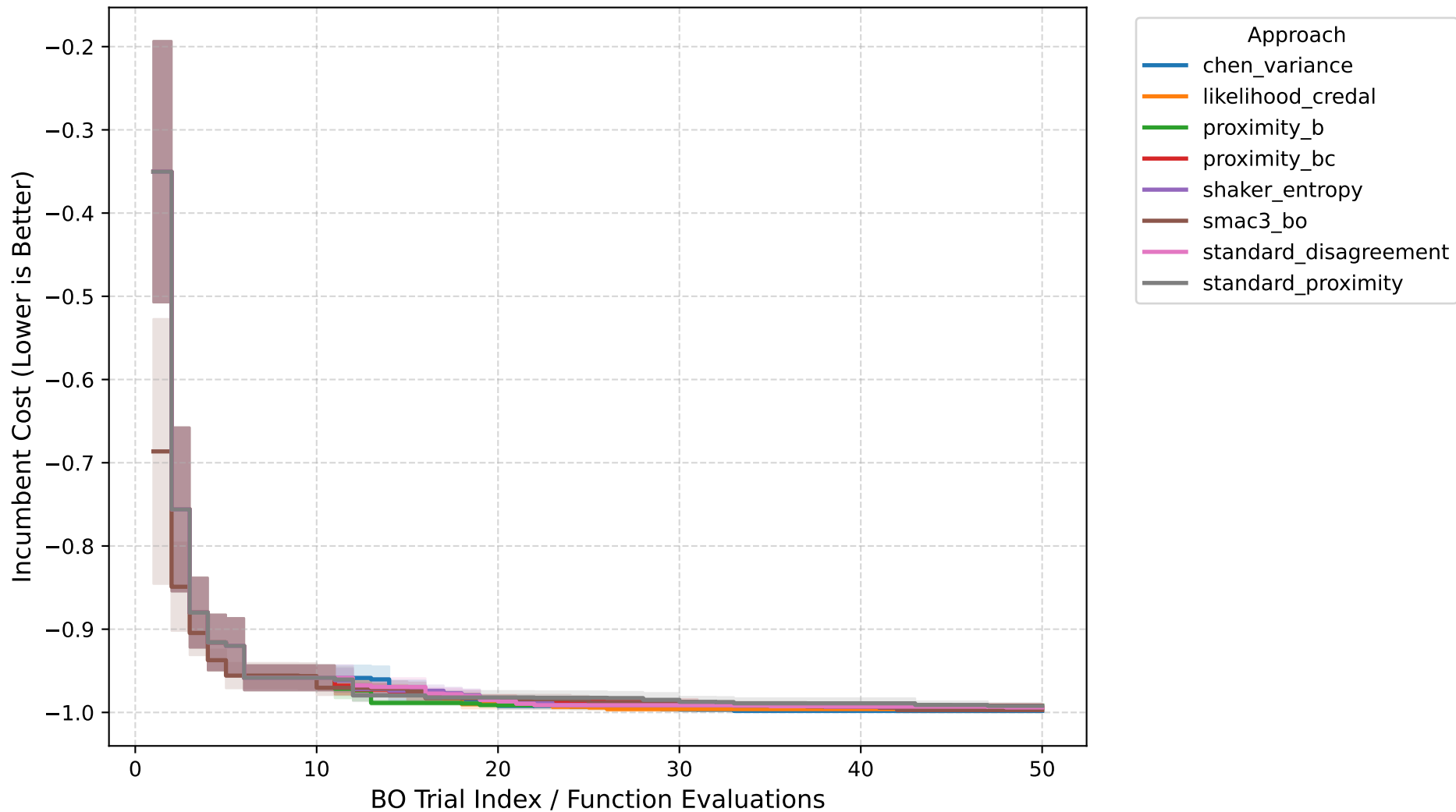
Anytime Performance: cfg_rbv2_xgboost_40499
