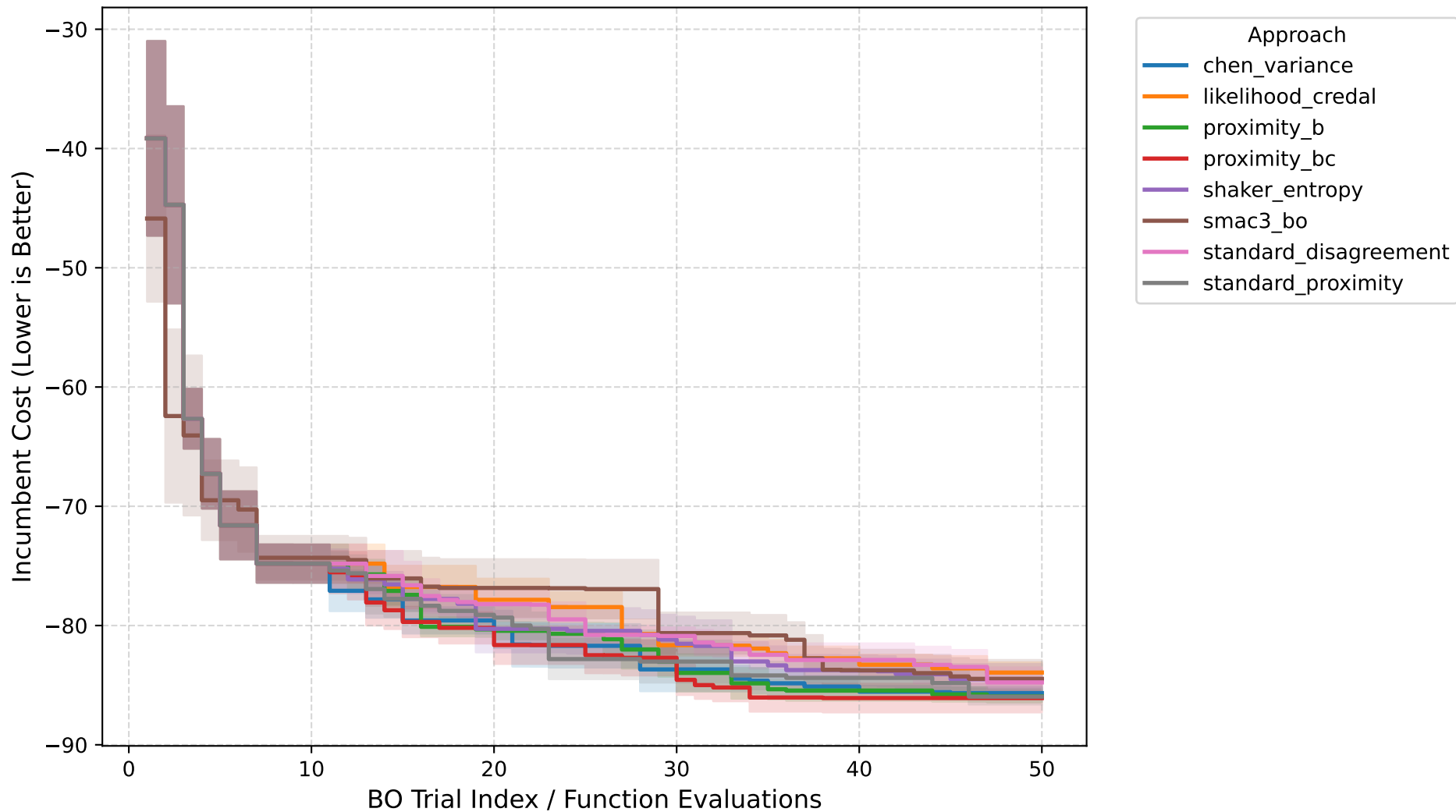
Anytime Performance: cfg_lcbench_167168
