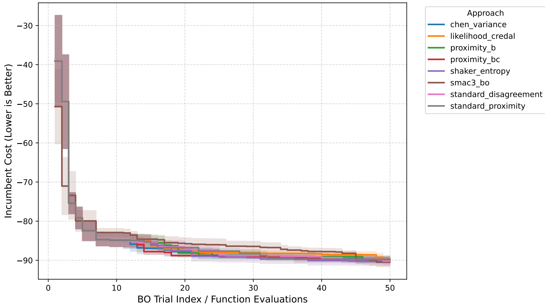
Anytime Performance: cfg_lcbench_189906
