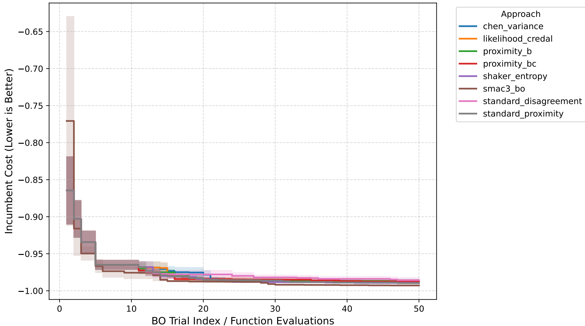
Anytime Performance: cfg_rbv2_ranger_42
