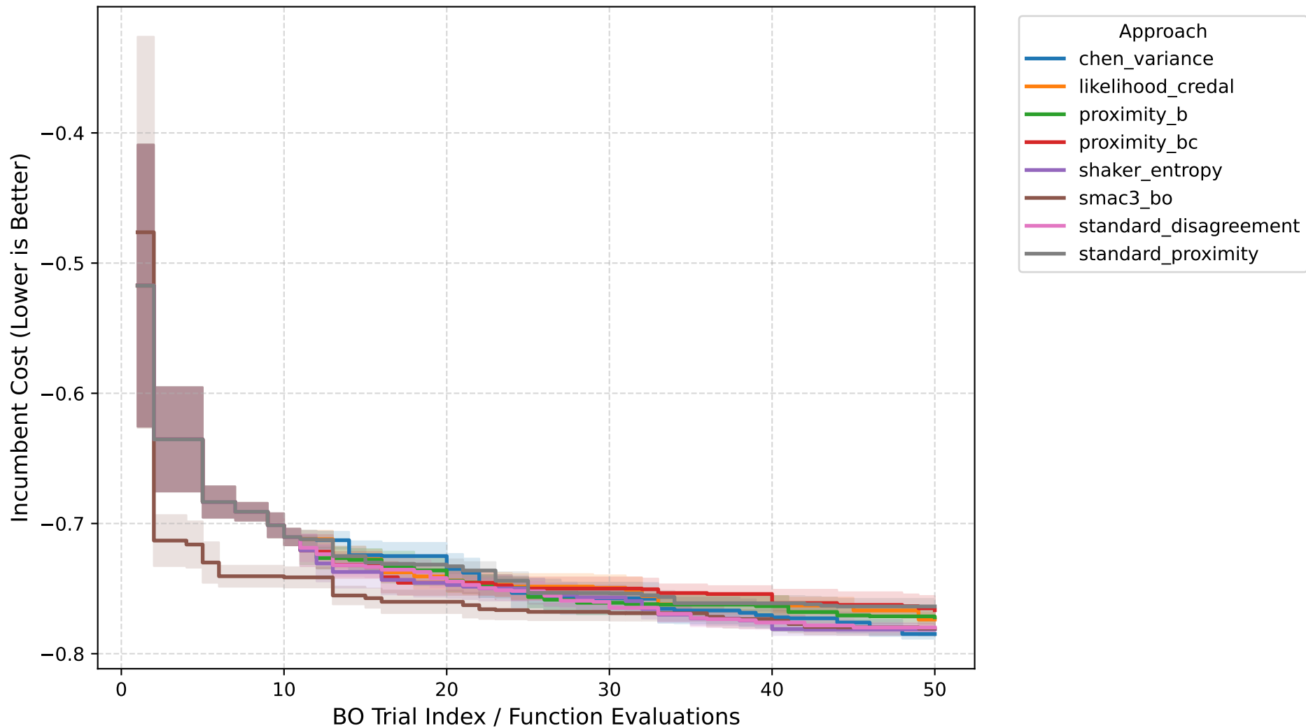
Anytime Performance: cfg_rbv2_rpart_14
