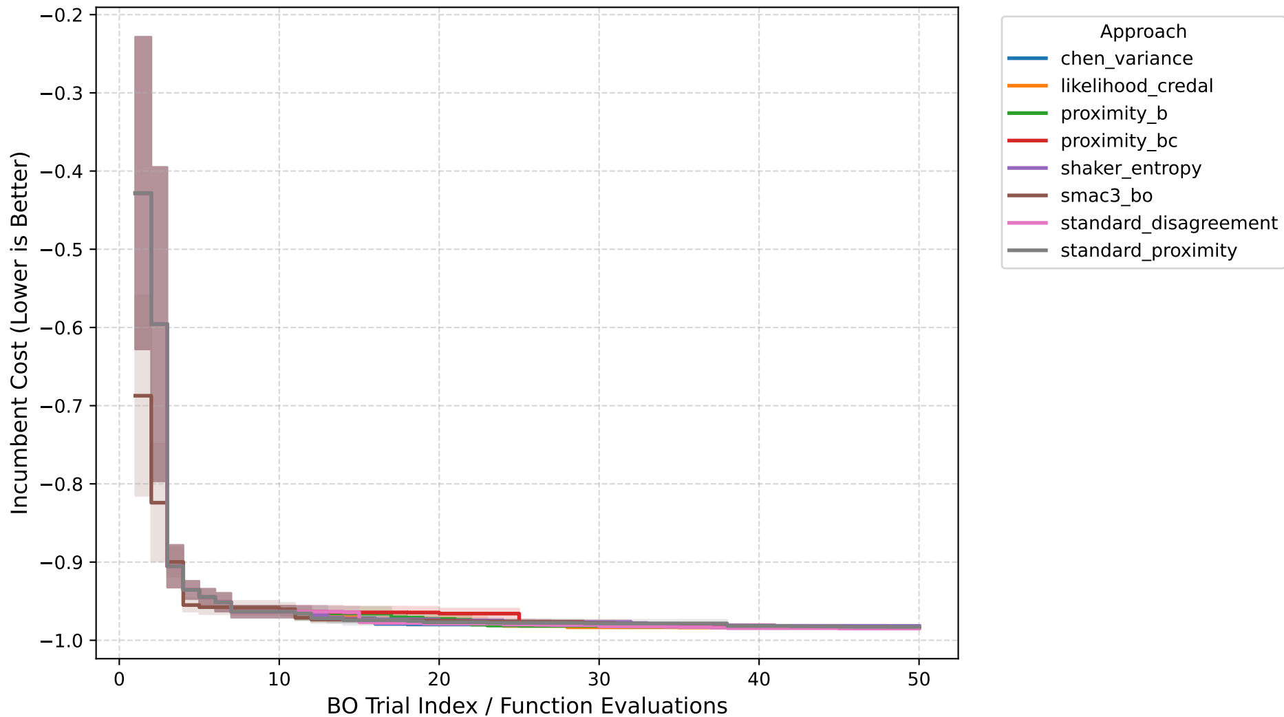
Anytime Performance: cfg_rbv2_xgboost_12
