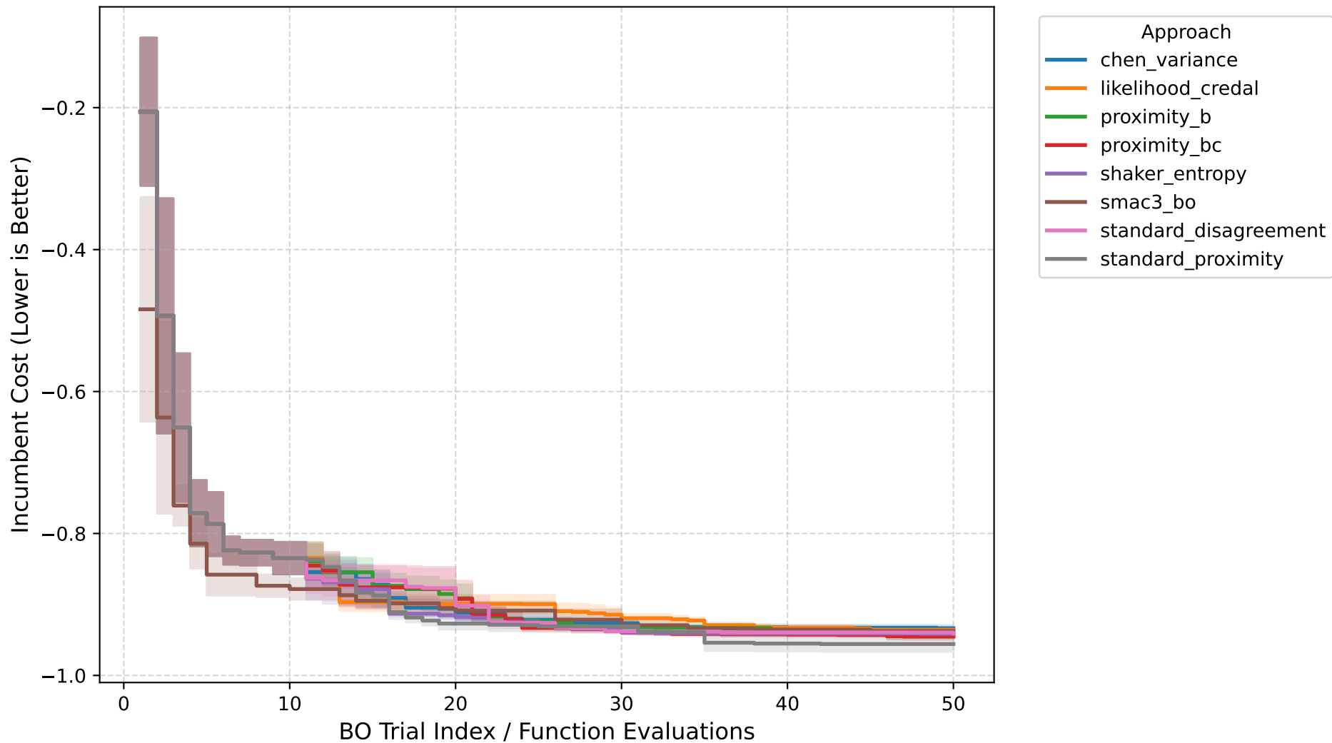
Anytime Performance: cfg_rbv2_xgboost_1501
