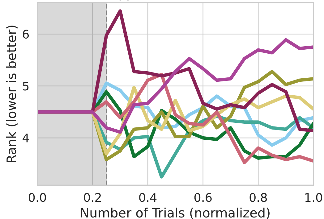
Task Type: blackbox, Set: dev
