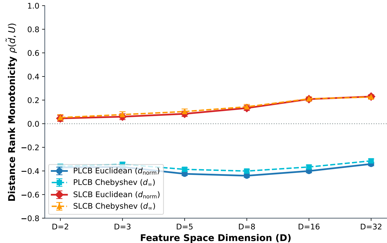
Surrogate Distance Sensitivity Scaling with Dimensionality
