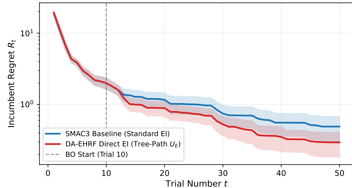
Sphere 2D ([-5, 5]^2)
