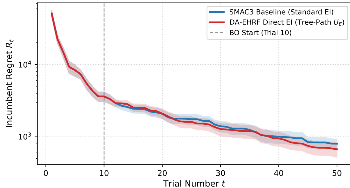
Rosenbrock 4D ([-5, 5]^4)
