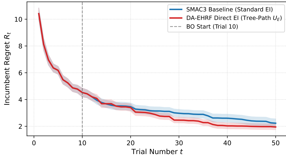
Sphere 2D ([-5, 5]^2)
