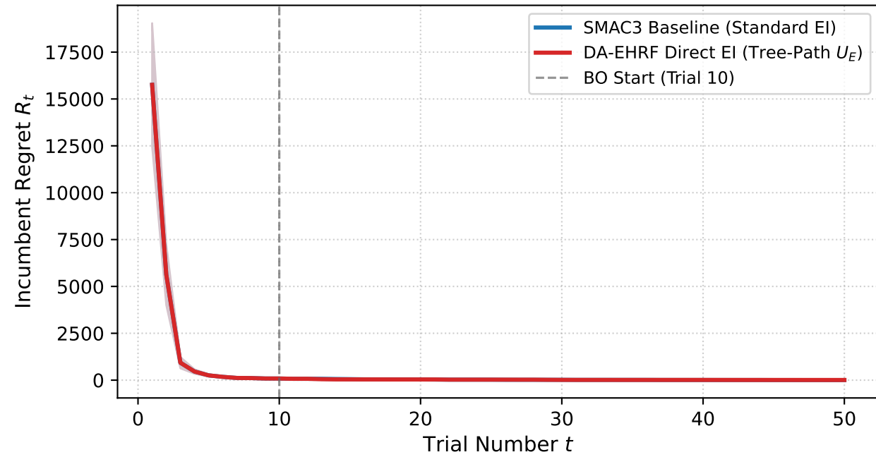
Rosenbrock 4D ([-5, 5]^4)
