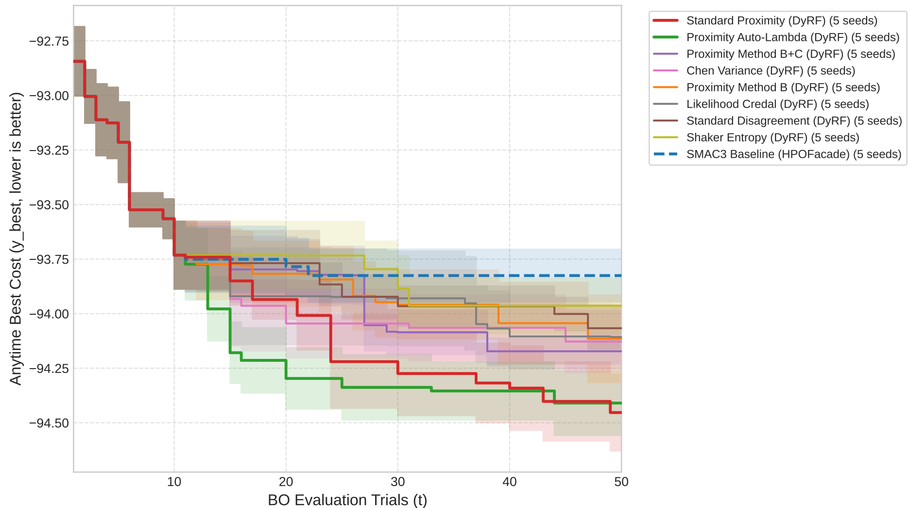
Anytime Performance on cfg_nb301_CIFAR10
