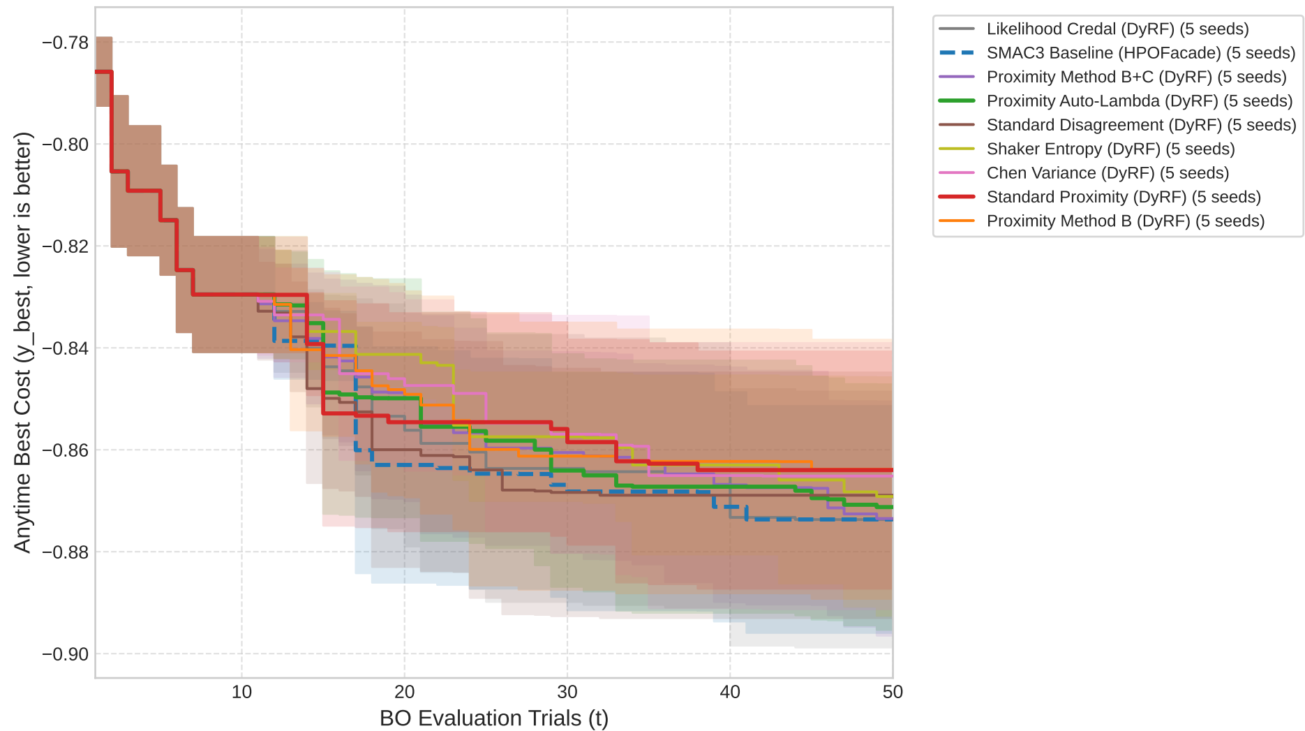
Anytime Performance on cfg_rbv2_super_1053
