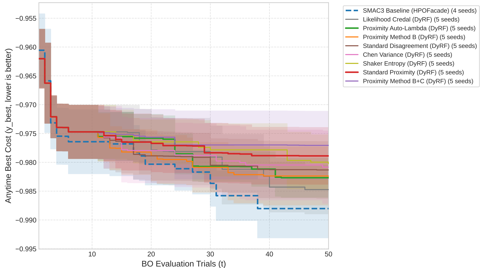
Anytime Performance on cfg_rbv2_super_1056
