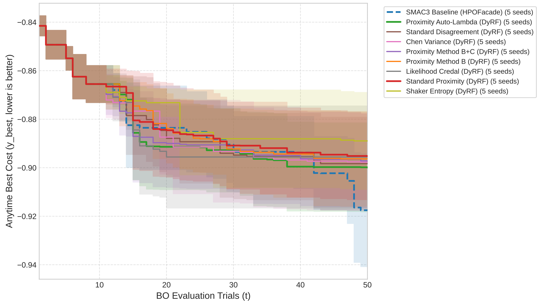
Anytime Performance on cfg_rbv2_super_1067
