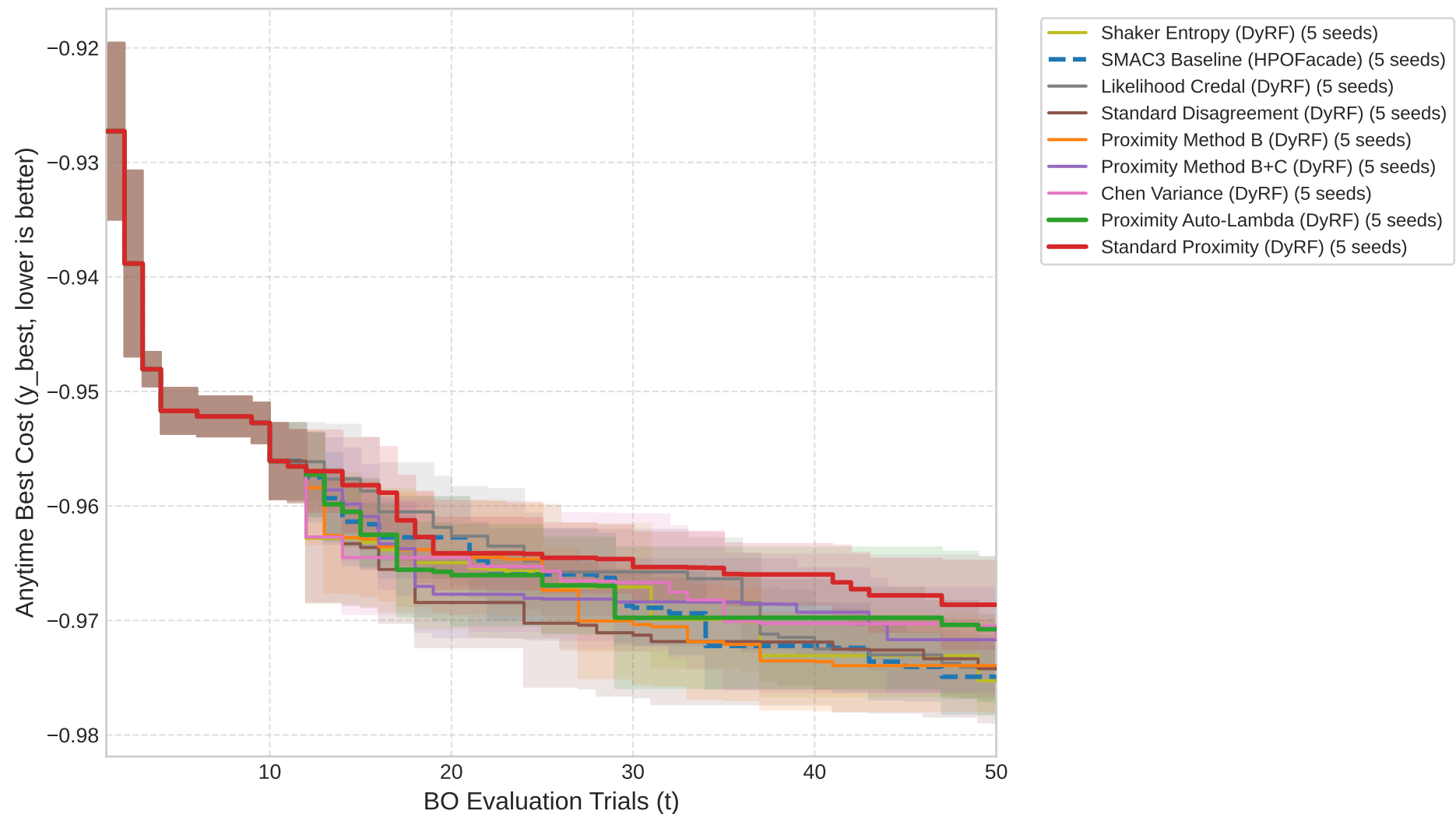
Anytime Performance on cfg_rbv2_super_1111
