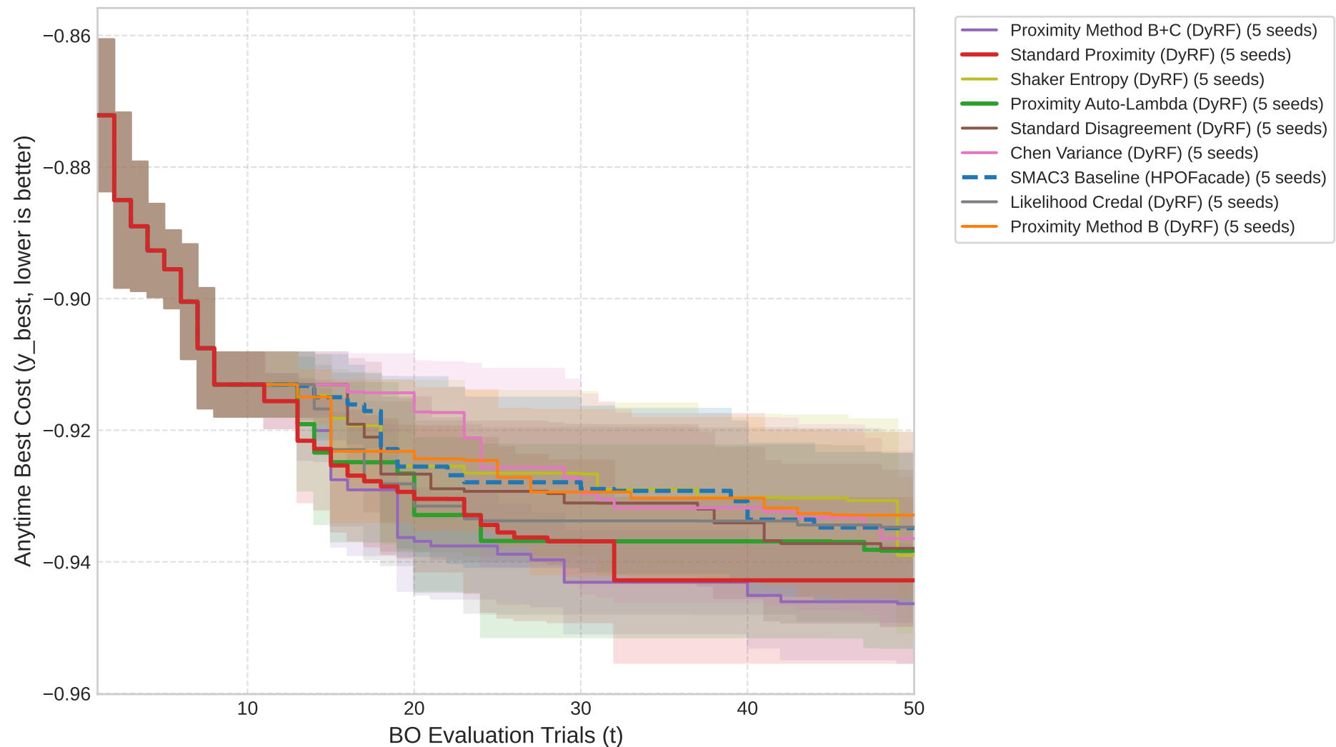
Anytime Performance on cfg_rbv2_super_1461
