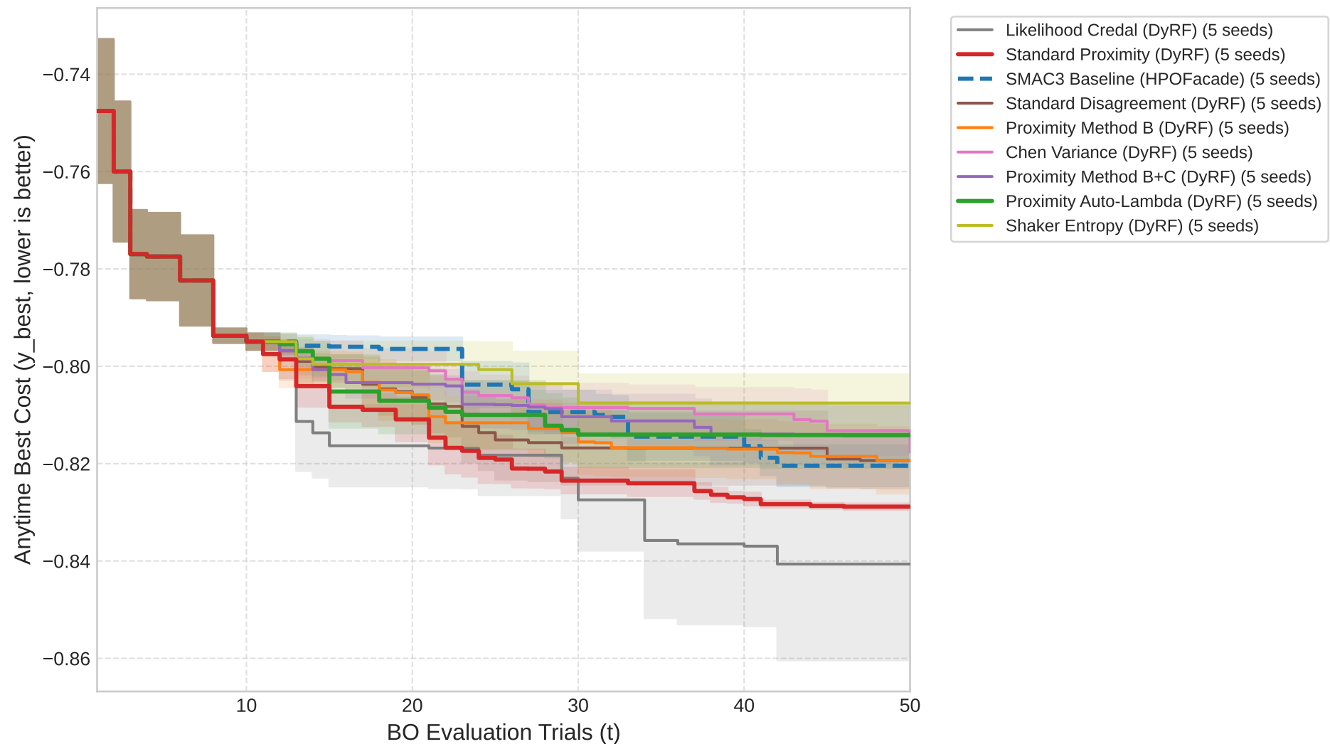
Anytime Performance on cfg_rbv2_super_1464
