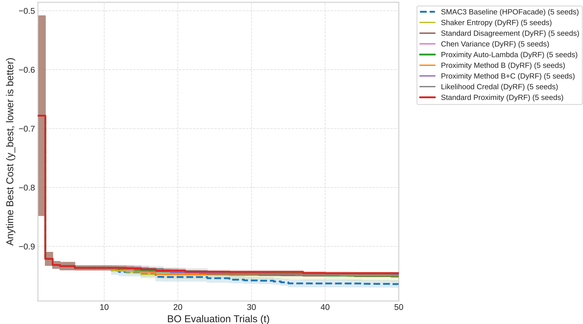
Anytime Performance on cfg_rbv2_super_1468
