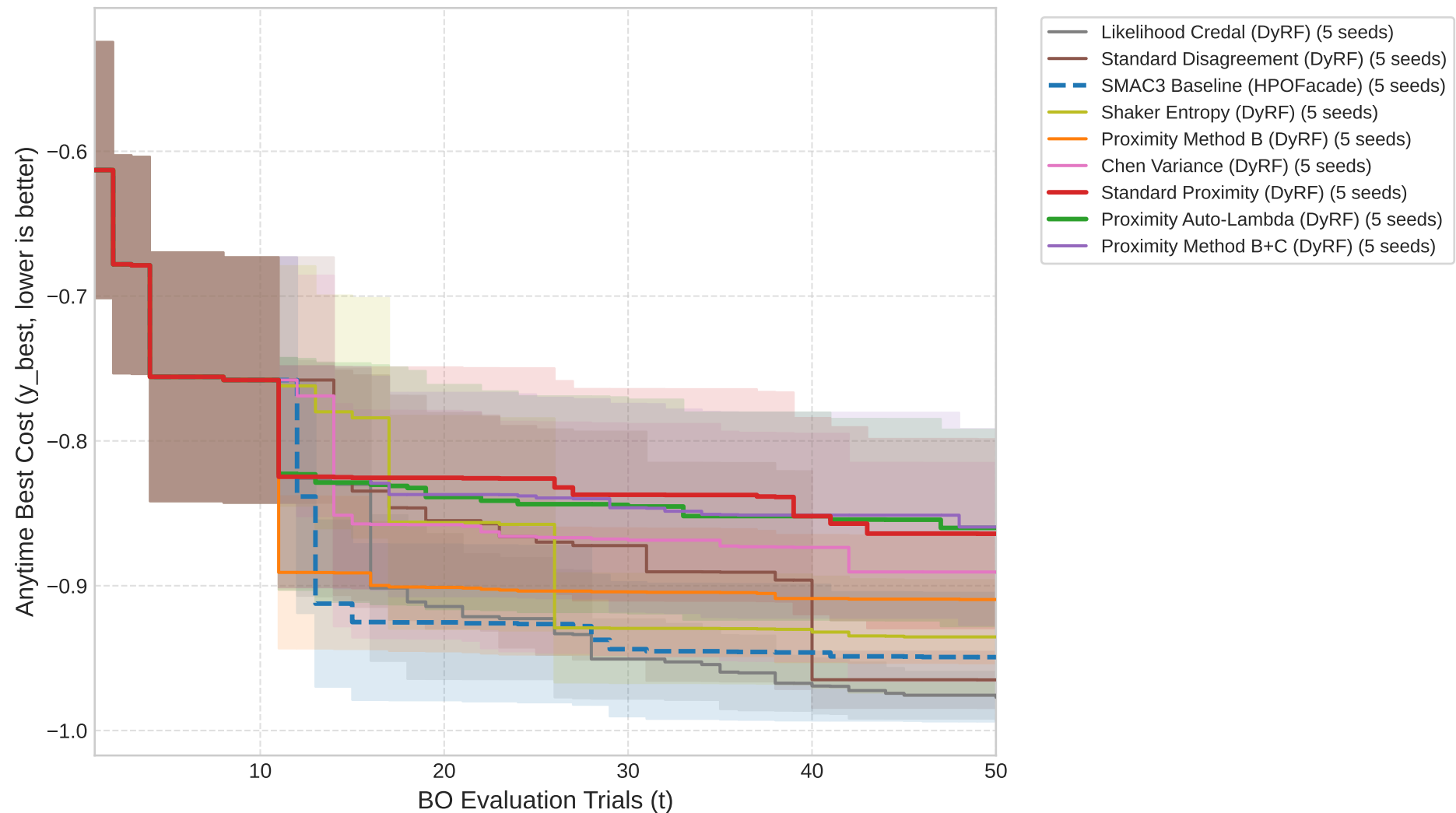
Anytime Performance on cfg_rbv2_super_1479
