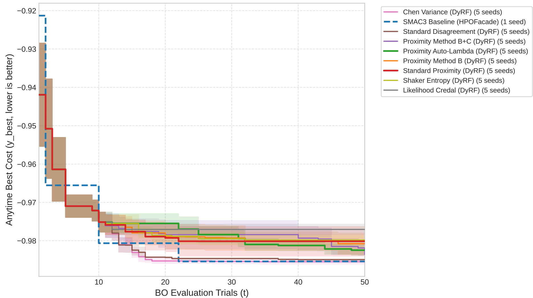
Anytime Performance on cfg_rbv2_super_15
