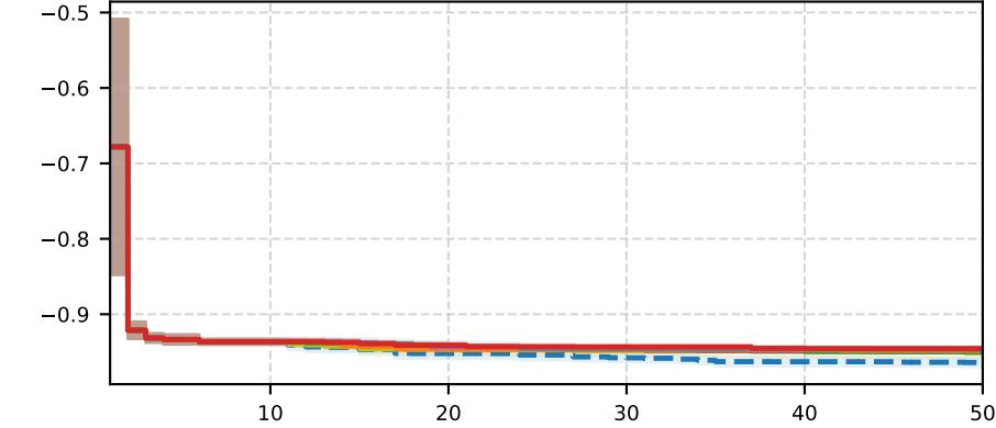
rbv2_1468
