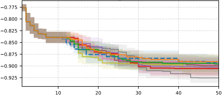
rbv2_1220
