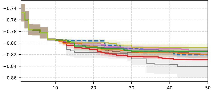
rbv2_1464
