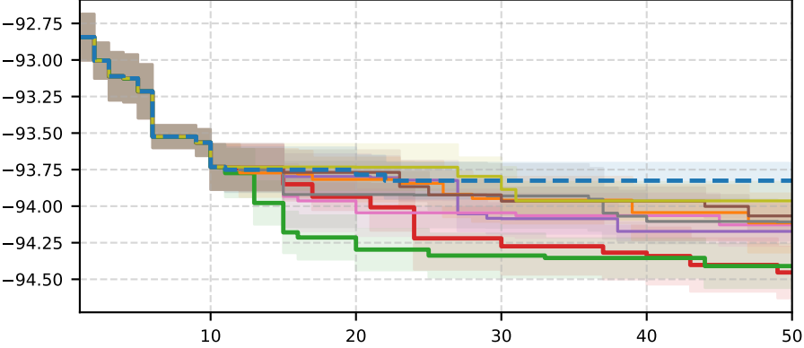
nb301_CIFAR10
