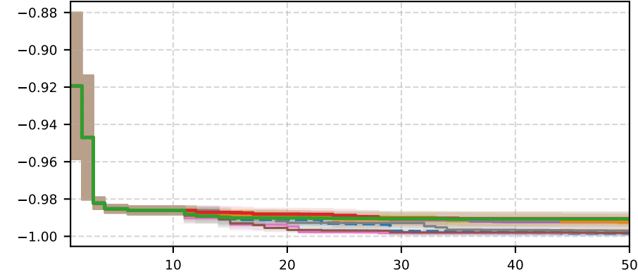
rbv2_1462
