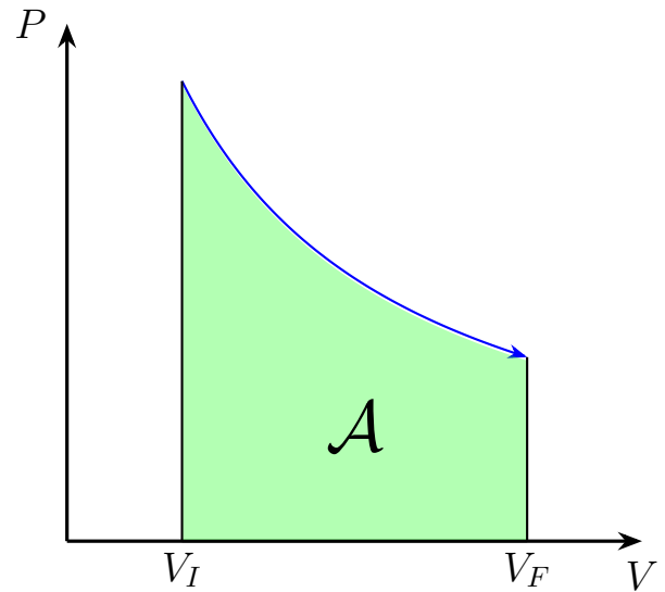
Figure B.6 – Hyperbole : P = \frac{nRT}{V}
