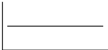
prior
