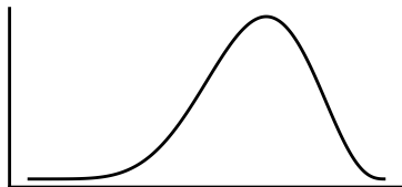
likelihood
