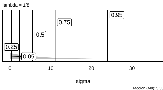
(e) lambda = 1/8
