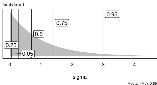
(b) lambda = 1
