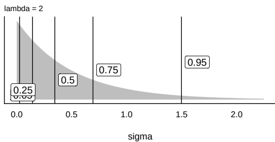
(a) lambda = 2
