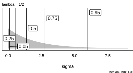
(c) lambda = 1/2
