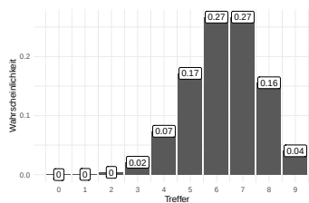
(b) n=9, p=.7
