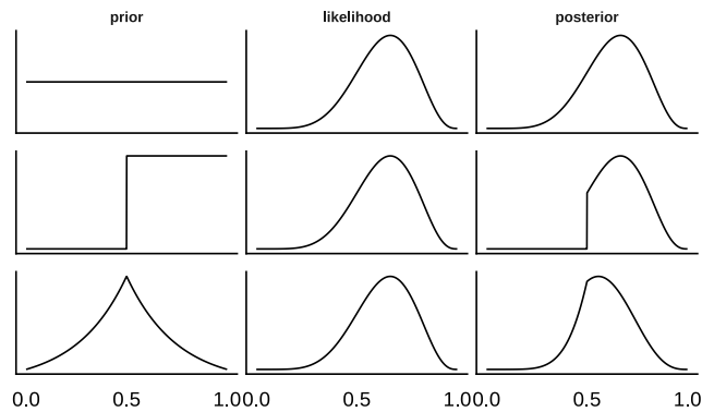
Abbildung 7.9: Prior mal Likelihood = Post
