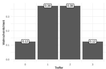
(a) n=3, p=1/2
