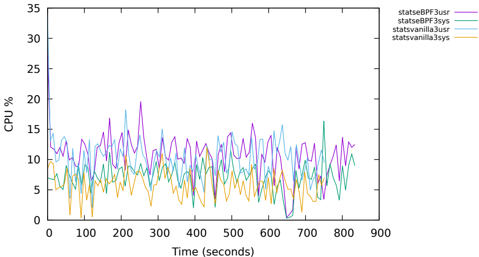
CPU usr + sys 3 replicas
