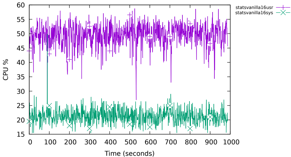
CPU usr + sys 16 replicas
