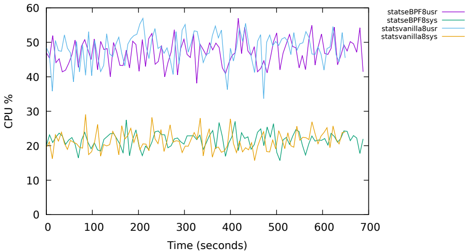
CPU usr + sys 8 replicas
