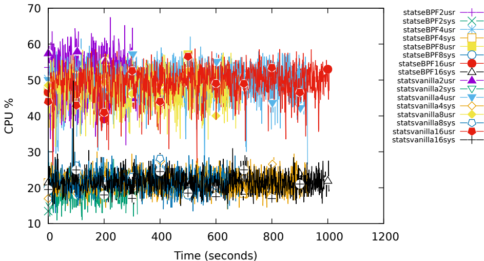
CPU usr + sys dstat
